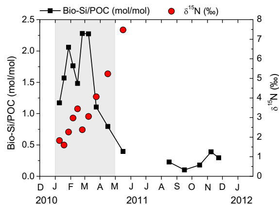
Fig. 3. Bio-Si/POC molar ratio (square; left y-axis) and \delta^{15}\text{N} (‰) values (circle; right y-axis) for available samples. The shaded area indicates the period of high particle flux (see text).
