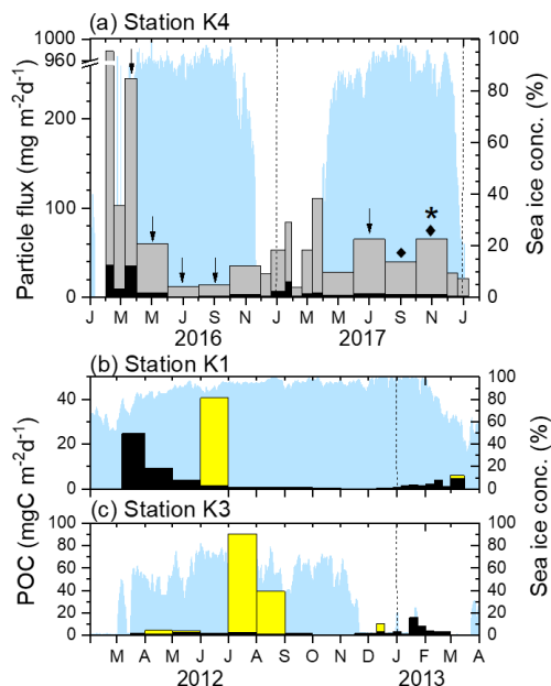
Figure 2. (a) Fluxes of sinking particles (gray bars) and POC (black bars) at Station K4. The tick marks on the x axis indicate the start of each month. The arrows, diamonds, and the star indicate the periods when worms, scallops, and the sea urchin were collected, respectively. (b) POC fluxes due to worms (yellow bars) and sinking particles (black bars) at Stations K1 and (c) K3. Note that the y axis scales differ. The dotted vertical lines denote the beginning of each year. The blue shading indicates the sea ice concentration. POC flux and sea ice data for Stations K1 and K3 were redrawn from Kim et al. (2019).
